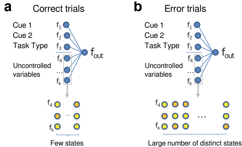
Figure S18: The toy model assumes that the recorded neurons receive inputs from four distinct upstream neural populations: three that represent the task-relevant variables, and one that represents the uncontrolled variables. a , In correct trials the patterns of activity encoding the uncontrolled variables can vary among a restricted set of states. b , In the error trials the set of possible values for the uncontrolled variables is assumed to be significantly larger, i.e. more variable, modeling the idea that the mental state of the animal is in one among numerous possibilities.
