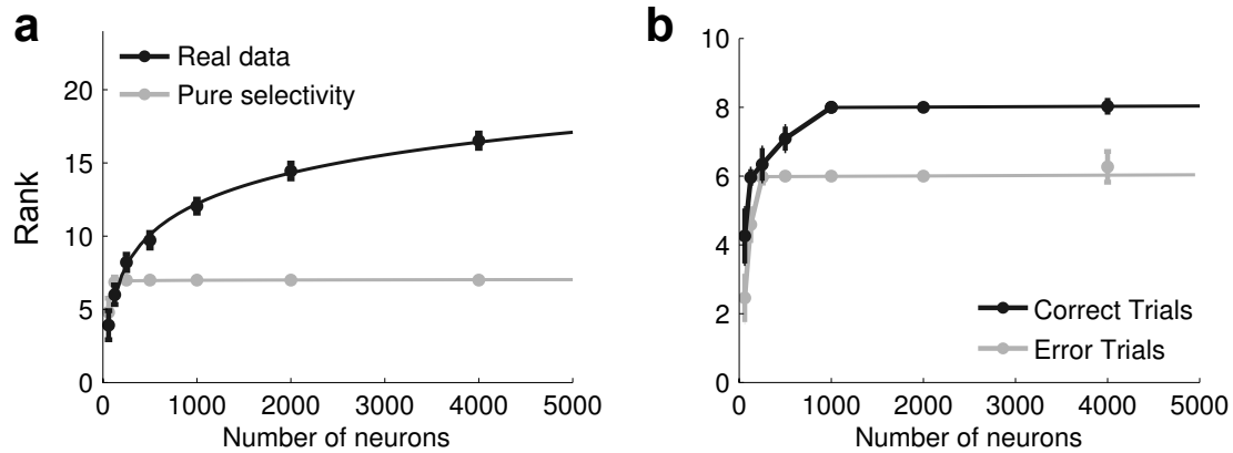
Figure S10: Number of significant principal components estimated as in [15] during a 800 ms time bin in the middle of the two-object delay epoch. a , Number of significant principal components (PCs) of the recorded PFC neural activity (black line), and the generated pure selectivity neurons (gray line). The recorded neural patterns display a dimensionality that is significantly larger than what would be expected under the assumption of the activity being primarily determined by pure selectivity to the aspects of the task, consistently with what we show in Fig. 4b. b , Number of significant PCs of the recorded PFC neural activity during the recall task for correct (black line) and error trials (gray line). Consistently with what we show in Fig. 5a the number of PCs during error trials is significantly lower than in correct trials.
