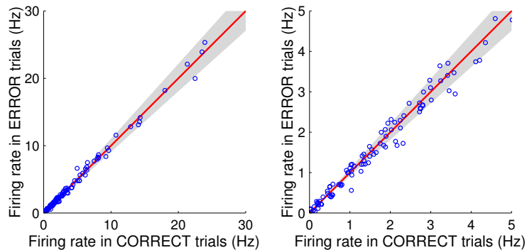
Figure S13: Overall firing rate in error trials as a function of firing rate in correct trials during the two-object delay epoch for the 121 neurons for which we have enough recall task trials to carry out the dimensionality analysis (at least 4 trials per condition). For these neurons we had on average \sim 208 correct trials and \sim 200 error trials per neuron. The panel on the right is a zoom-in on the panel on the left in a range between 0 and 5 Hz. The red diagonal indicates the points where the graphed dots should fall in the case of exactly equal firing rates in correct and error trials. The gray shading indicates the deviations away from the diagonal that can be explained by finite sampling of underlying Poisson spike counts (standard error of the mean).
