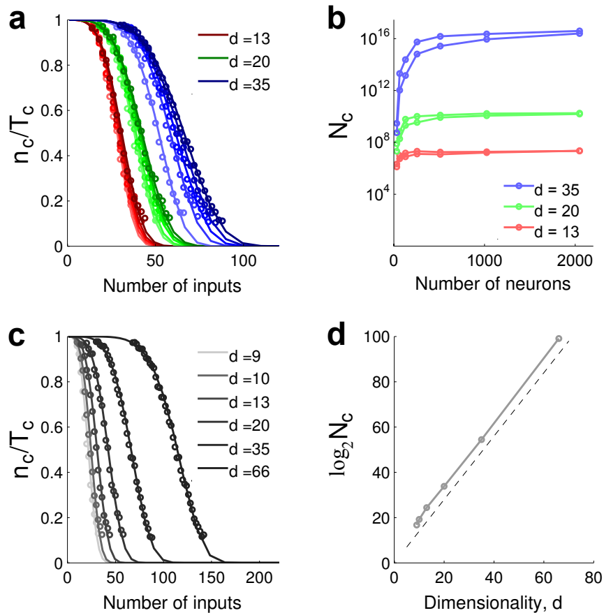
Figure S6: Relation between input vectors dimensionality and number of implementable classifications. a , Fraction of correctly implementable binary classifications as a function of the number of input patterns for different dimensionalities ( d = 13, 20, 35 ) and different number of neurons (darker curves correspond to more neurons). b , The advantage of increasing the number of neurons saturates very quickly and at a level that does not depend on the noise intensity. The saturation level only depends on the dimensionality of the inputs d . c , Same as a , but at saturation (i.e. with enough neurons to reach saturation), for different input dimensionalities. d , Total number of implementable binary classifications N_c as a function of input dimensionality. N_c grows exponentially with d . The dashed line correspond to an exponential growth with exponent of 1.4, slightly lower than the theoretical one of 2 obtained in the noiseless uncorrelated case [33].
