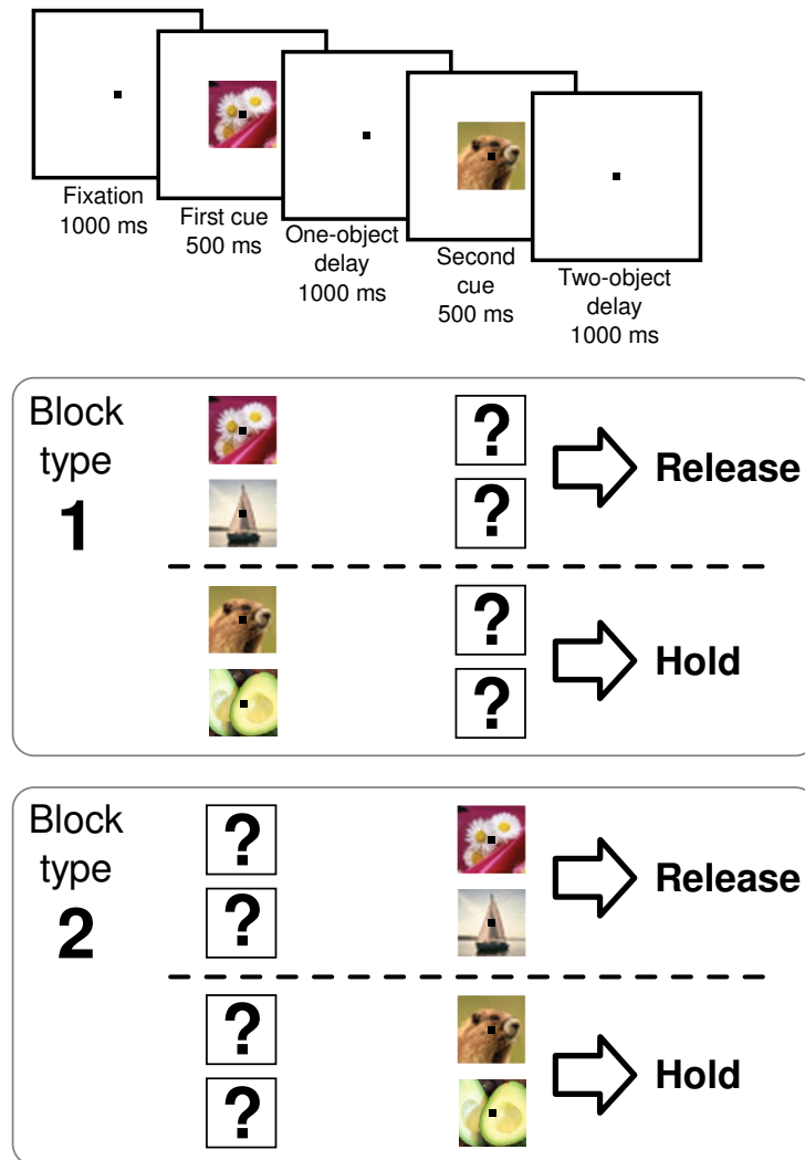
Figure S8: A hypothetical virtual task that uses the same elements of the sequence learning task. The task type variable of the original task is used to encode the currently active rule (look at cue 1 and ignore cue 2, or look at cue 2 and ignore cue 1). If the relevant cue is either object A or B the subject then has to release a bar, and is required to hold the bar if the relevant cue is either object C or D.
