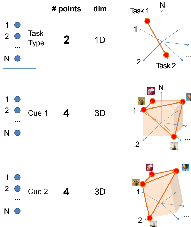
Figure M1: Expected dimensionality for neural representations with pure selectivity neurons in the memory sequence task. Filled blue circles represent neurons. Each population of neurons encode only one task-relevant aspect (pure selectivity). From the top, there are first the neurons encoding task type, then cue 1 and cue 2. Each population has size N and patterns of activity can be represented as a points in an N -dimensional space (red circles). However, as there are only two possible task types, the patterns of activity generated by recall (task 1) and recognition task (task 2) representations lie on a line (a vector space of dimensionality 1). Indeed, there is always a line going through the two points (red), regardless the specific representation of the two tasks. Analogously, the patterns of activity generated by cue 1 and cue 2 pure selectivity neurons lie in a space of dimensionality 3, as there are only 4 possible objects). The dimensionality of the neural representations then equals the dimensionality of the vectors spaces defined by the patterns of activity, to which we have to add one in order to take into account the additional degree of freedom given by the displacement of the patterns of activity from the origin.
