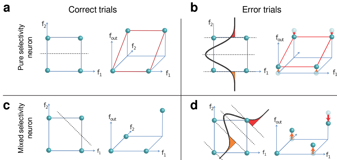
Figure S19: The variability in the mental states leads to a reduction of the signal and an increase in noise. Non-linear mixed selectivity neurons are more sensitive to these changes. a,c , Left: Diagrams representing the input space for pure/non-linear mixed selectivity neurons in the correct trials. f_1 and f_2 are two inputs representing task-relevant variables. Each point on the plane represents an input pattern of activity. The separating dashed line divides the inputs which are below threshold from those that are above threshold. Assuming that both f_1 and f_2 are either high or low, there are 4 possible inputs, here represented by spheres. a,c , Right: the input-output relation. f_{out} is the activity of a neuron receiving input from f_1 and f_2 . The output is a linear function of the inputs in a , for a pure selectivity neuron (see the plane delineated by the red segments), and non-linear in c . b,d , Same as in a,c , but now in the error trials, in which the inputs encoding the uncontrolled variables generate noise. The orientation of the linear separator depends on the synaptic weights from the two inputs encoding the task-relevant variables. Its position depends on both the activation threshold and on the noisy input generated by the other neurons, those that encode the uncontrolled variables. The position of the separating line is now stochastically distributed across trials (Gaussian curve in the left panel). There is some fraction of trials in which the dashed lines moves across one of the input points. The probability that this happens is the colored area under the distribution. The probability that the inputs are still generating the same output as in the correct trials is an integral over the interval between the colored areas. The diagram on the right represents geometrically the effect of the noise as an average “flattening” of the combined input-output activity patterns. The effects of noise on pure and non-linear mixed selectivity neurons are qualitatively the same, but quantitatively different for pure and non-linear mixed selectivity neurons, as described in the text.
