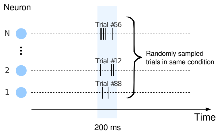
Figure M7: Generation of pseudo-simultaneous population activity patterns used to train and cross validate the population decoder. We generate a pattern of activity corresponding to a given condition c by randomly sampling for every neuron i a trial n_i^c recorded in condition c . We compute the spike count in such trial in 200 ms bins.
