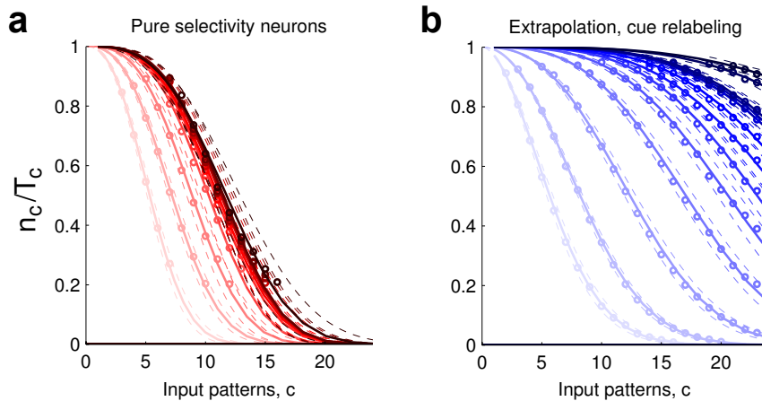
Figure M8: Fraction of implementable binary classifications n_c/T_c as a function of the number of input patterns c among the possible 24 conditions that are classified. Different curves correspond to different number of neurons representing the inputs (darker curves correspond to increasing number of neurons). The firing rate activity of the neurons is computed over the 800 ms in the middle of the second-object delay period. a , Fraction of implementable binary classifications n_c/T_c with a test error of at most \theta_{error} = 0.2 . The neural population over which the inputs are sampled are pure selectivity neurons generated as explained in Supplementary Methods M.4. b , Same as in a for recorded PFC data after extrapolation to larger number of neurons by relabeling object identities as explained in Supplementary Methods M.6. Data points are fitted with the Weibull curves y(c) = \exp(-c^\alpha/\beta) .
