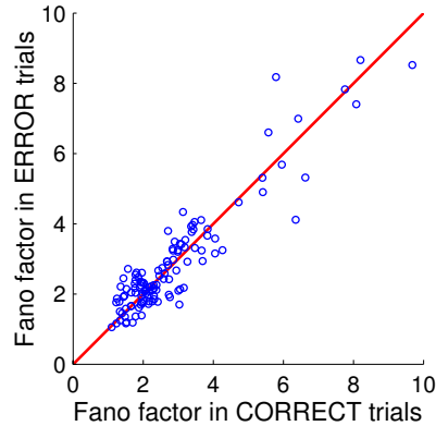
Figure S14: Comparison of the average Fano factor during correct and error trials in the two-object delay epoch of the recall task. Every dot in the graph indicates the Fano factor of a recorded neuron in the two-object delay epoch averaged across conditions computed during correct trials and plotted against the same quantity during error trials. The figure does not show any large or systematic deviation from the diagonal, and a Wilcoxon rank-sum test indicates that the distribution does not change significantly between correct and error trials (Wilcoxon rank-sum test, p > 0.6 ).
