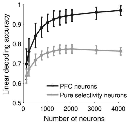
Figure S9: Cross-validation performance of a linear decoder trained on a classification task that is equivalent to the virtual task illustrated in Fig. S8. Training such a decoder can be thought of as training a neuronal response function to execute the motor output that is necessary for the task. The curves show the cross-validated performance as a function of the number of neurons for two types of representations of the input. The black curve indicates the performance when the input population is composed of the recorded PFC neurons, while the gray curve shows the case where the input population is composed of pure selectivity neurons. Consistently with what shown in Figs 4a,b, the performance of the binary function on the pure selectivity neurons is significantly worse than when the input is represented by the recorded data.
